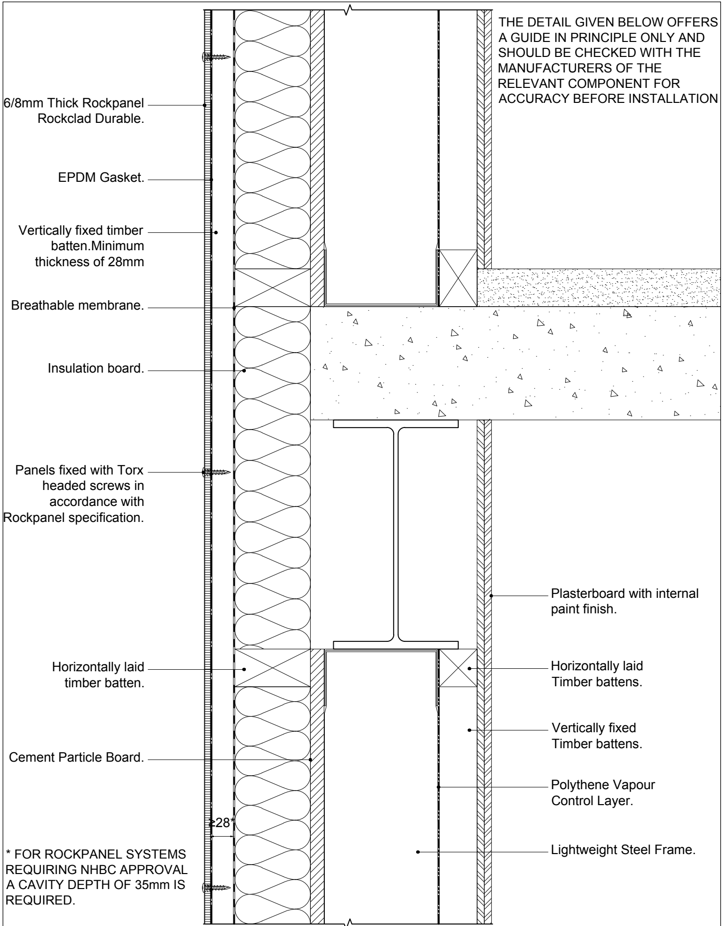
DETAIL 8 - ROCKCLAD DURABLE VERTICAL SECTION TIMBER SUBSTRUCTURE TO STRUCTURAL STEEL WITH LIGHT STEEL FRAME.
